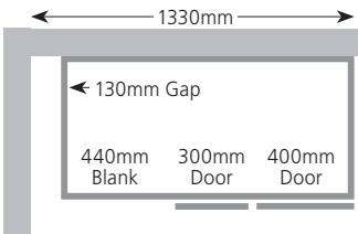
Full Height Door CB126FF Drawer Line CB126DF
